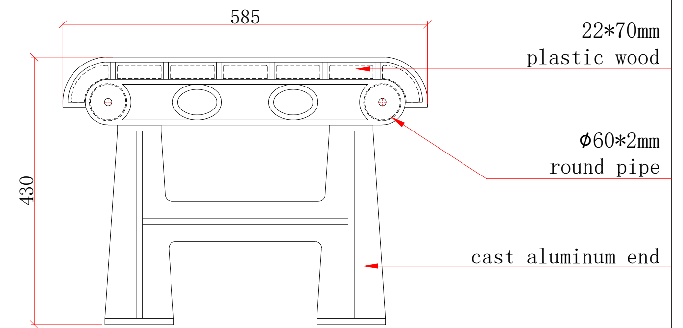
SIDE VIEW
