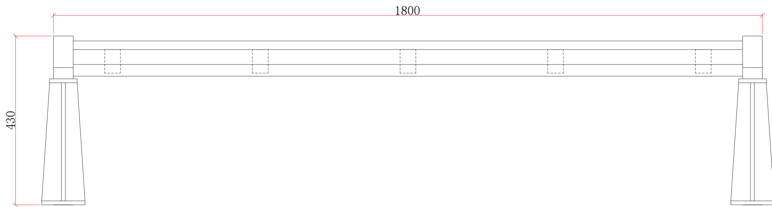
FRONT VIEW
